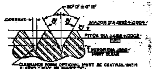
ENLARGED SECTION - THREAD PROFILE A SCALE: NONE
